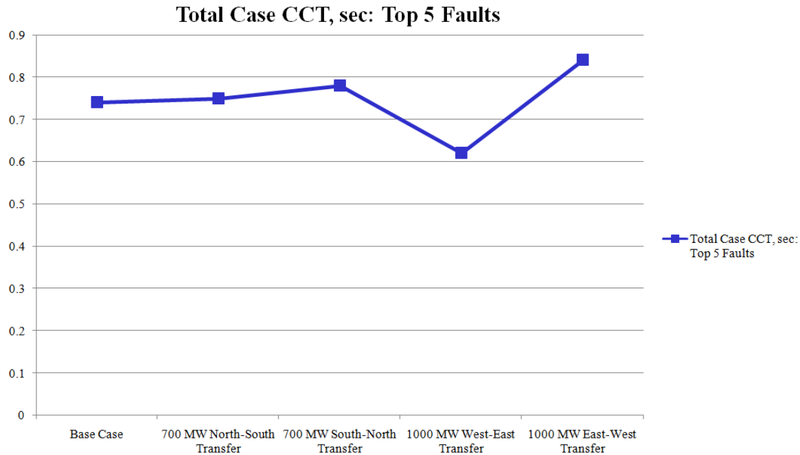
Figure 5-15. Total Case CCT for the Base Case and Transfer Cases
