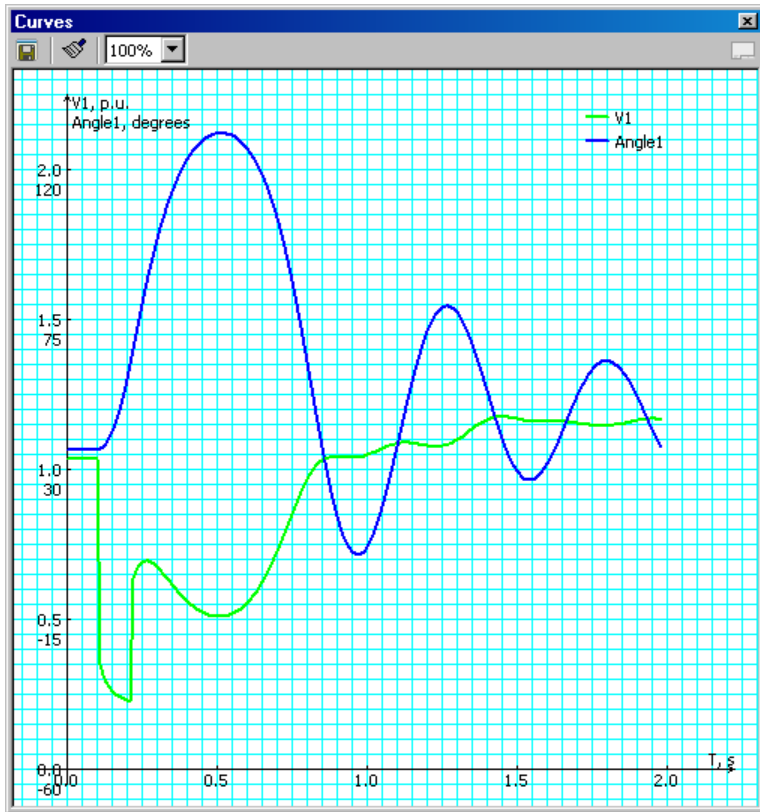
Figure 6-21. Fault at Bus # 115.0 Clears in 0.12 sec
