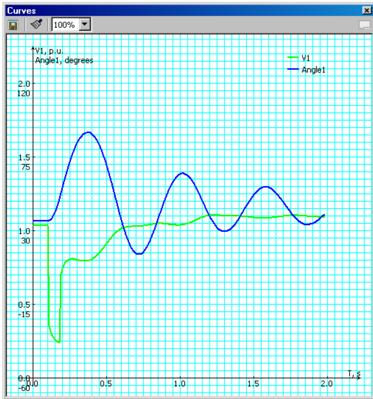
Figure 6-20. Fault at Bus # 115.0 Clears in 0.08 sec
