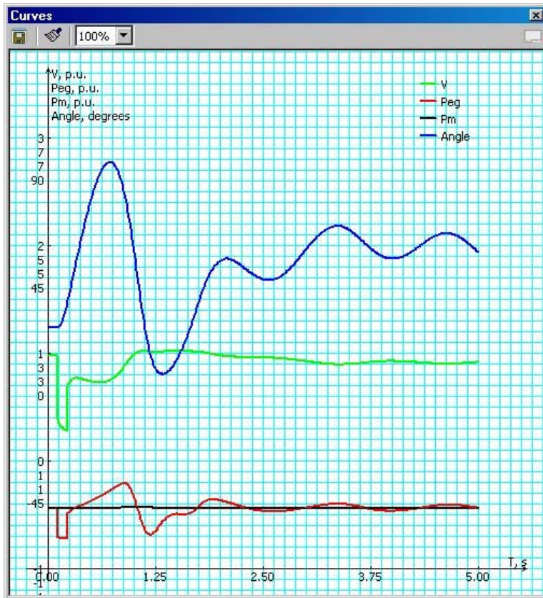
Figure 5-7. Fault at Bus # [redacted] Clears in 0.12 sec
