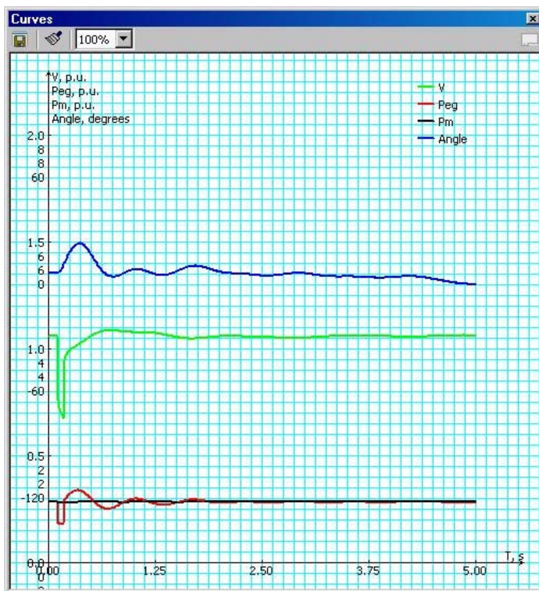
Figure 5-10. Fault at Bus # [redacted] Clears in 0.08 sec
