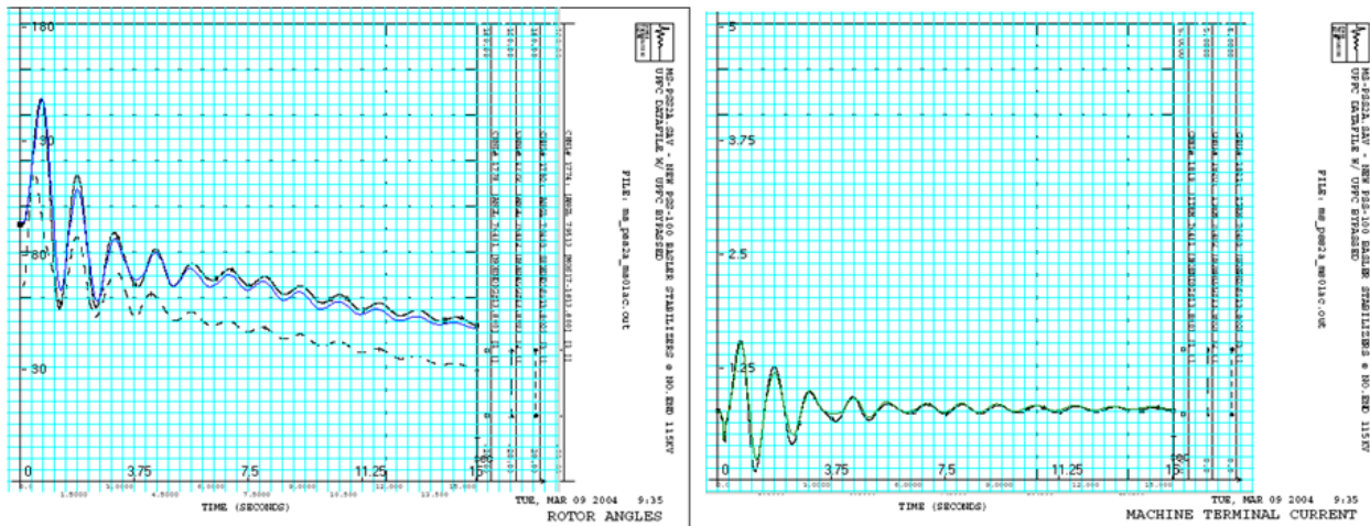
Figure 8-4. POM-TS and PSS/E Results
