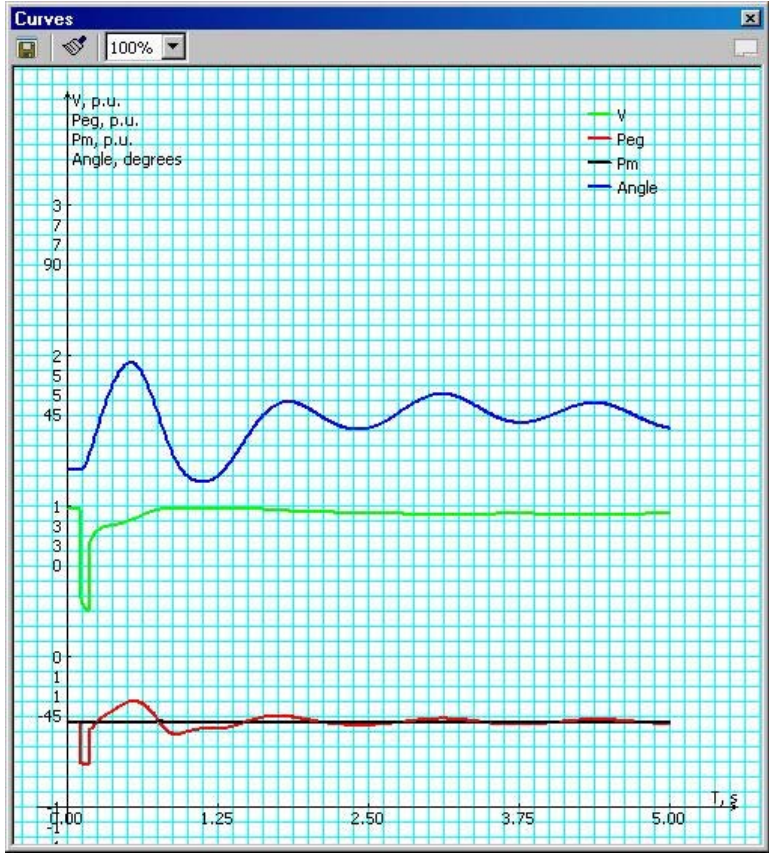
Figure 5-6. Fault at Bus # [redacted] Clears in 0.08 sec
