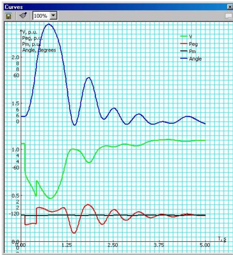
Figure 5-11. Fault at Bus # [redacted] Clears in 0.27 sec
