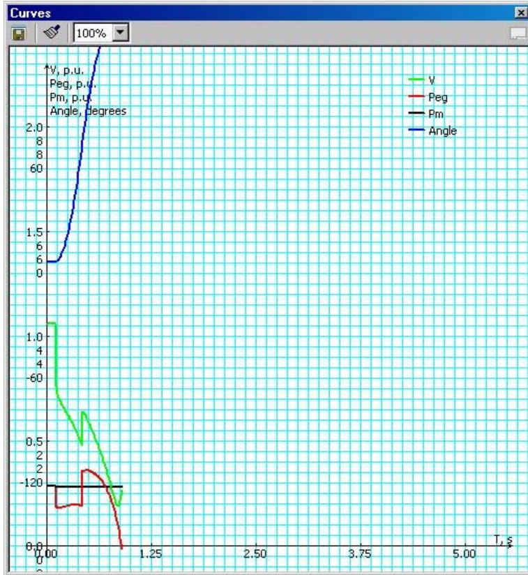
Figure 5-12. Fault at Bus # [redacted] Clears in 0.28 sec
