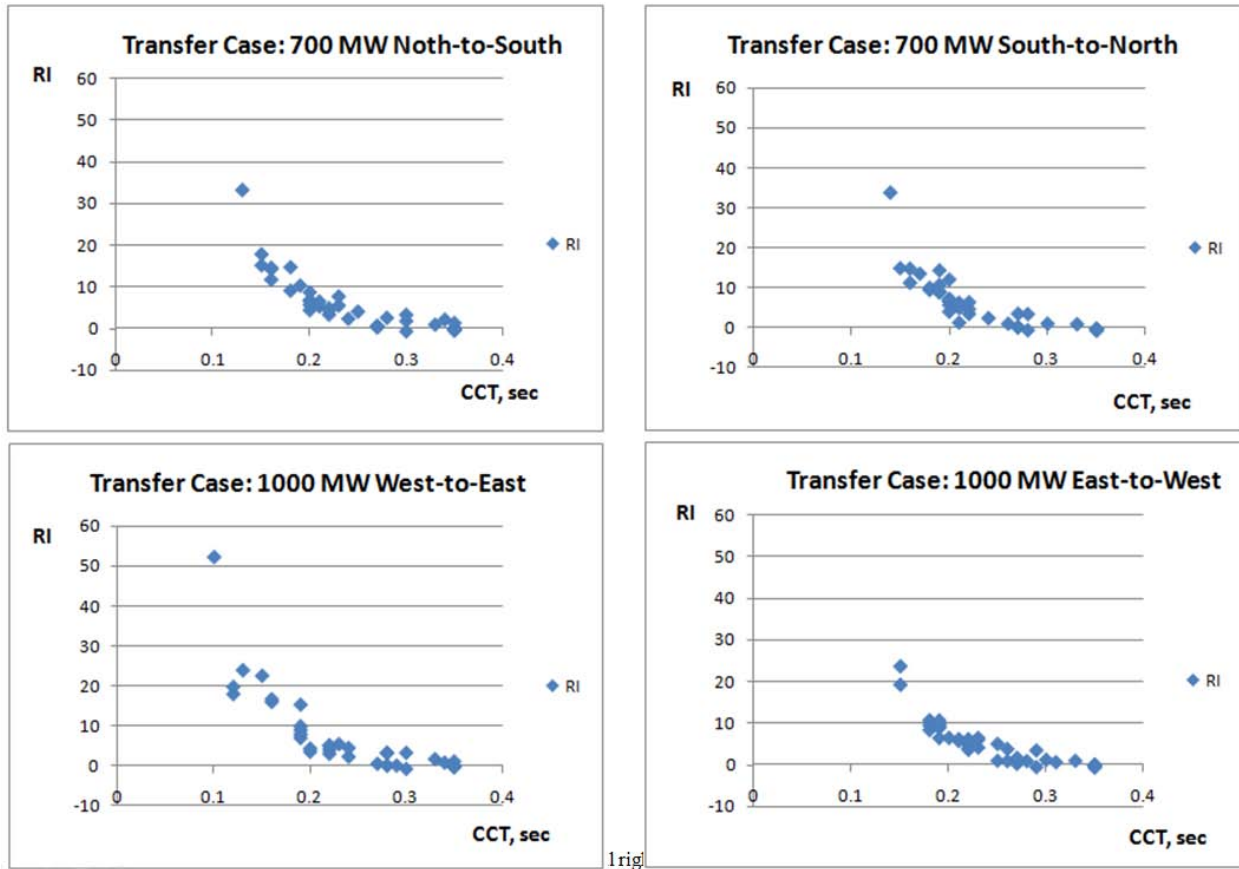
Figure 5-13. Distribution of the Ranking Index by the Critical Clearing Time for Transfer Cases
