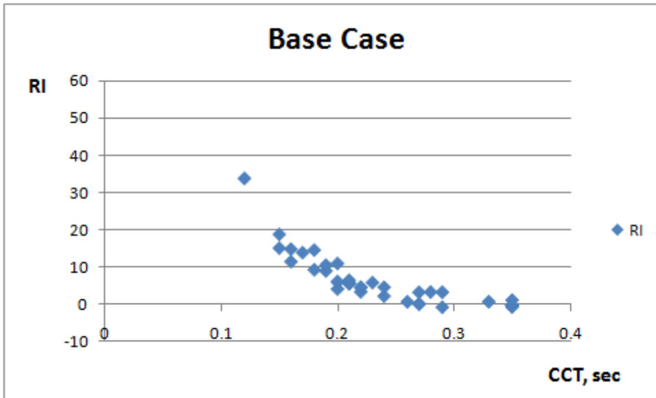
Figure 5-4. Distribution of the Ranking Index by the Critical Clearing Time for the Base Case
