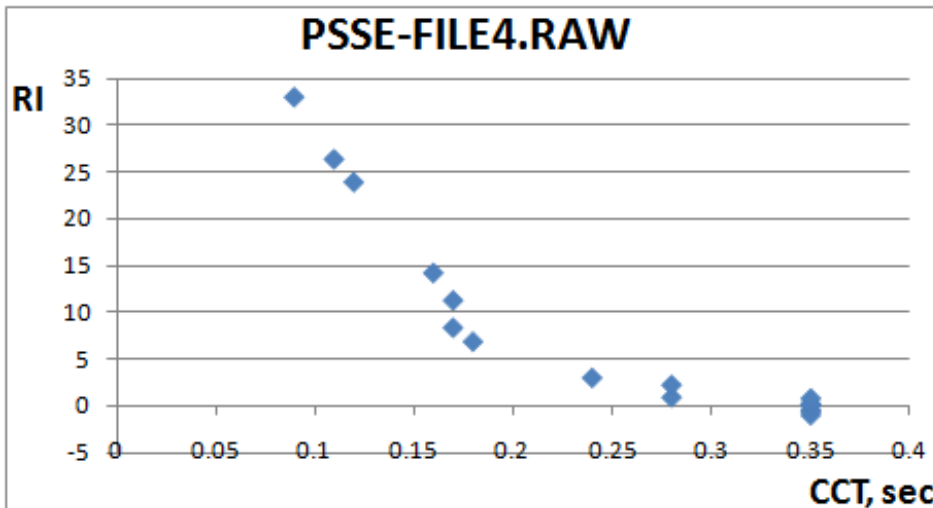
Figure 6-29. Distribution of the Ranking Index by the Critical Clearing Time for Case “PSSE-FILE4.RAW”
