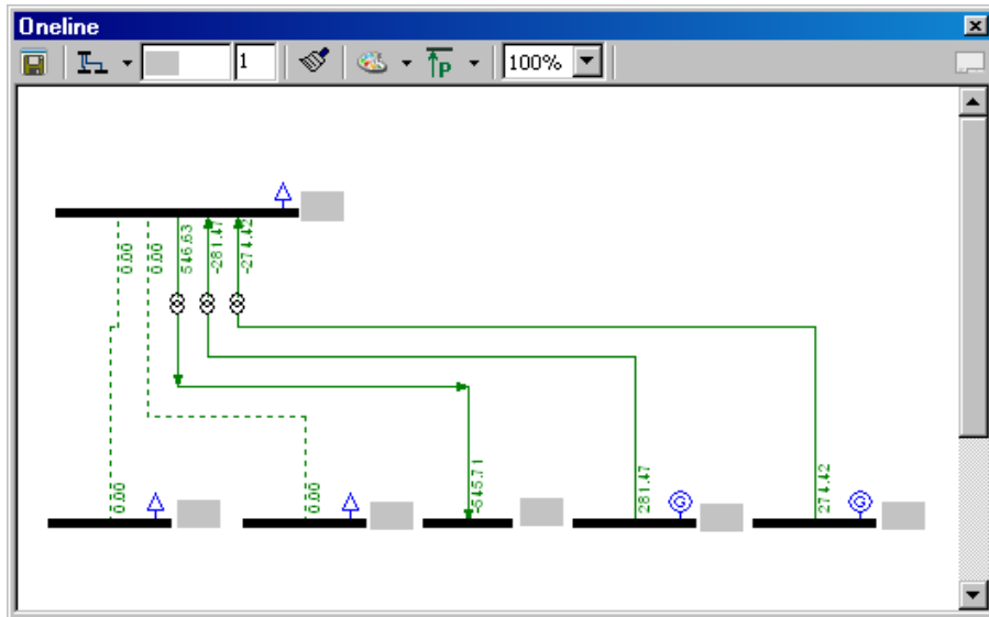
Figure 6-23. Online Diagram for Bus # 138.0
