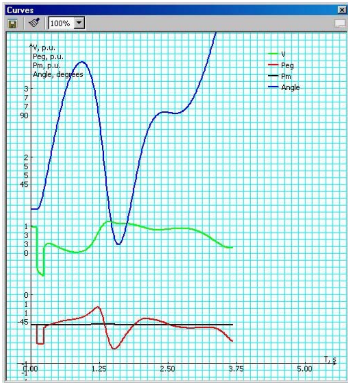
Figure 5-8. Fault at Bus # [redacted] Clears in 0.13 sec
