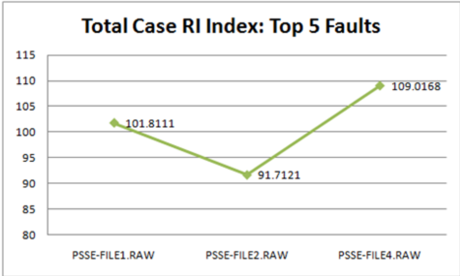
Figure 6-30. Total Case RI for EMS Cases
