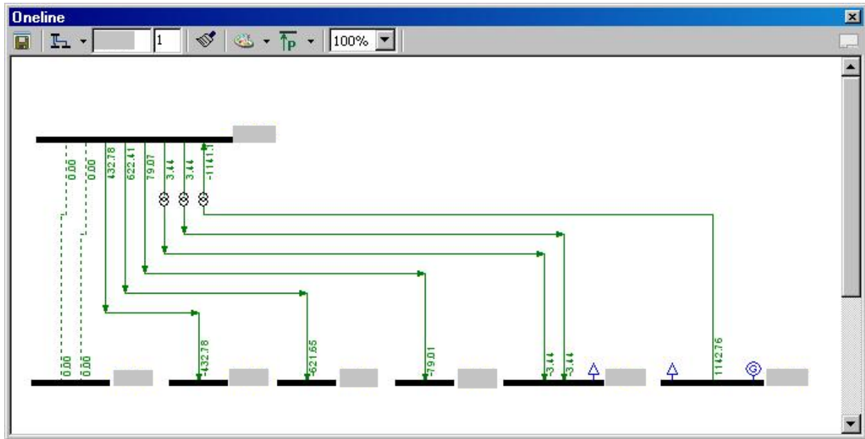
Figure 5-5. Oneline Diagram for Bus # [redacted]
