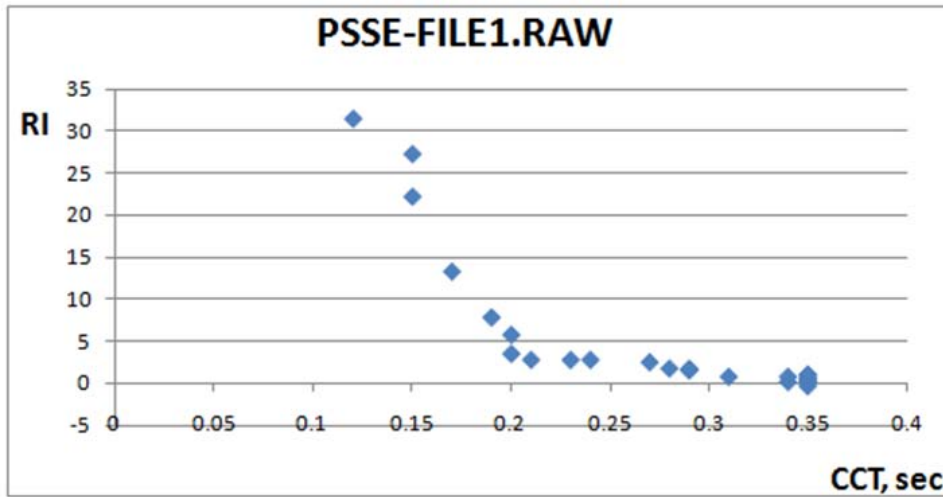
Figure 6-17. Distribution of the Ranking Index by the Critical Clearing Time for Case “PSSE-FILE1.RAW”
