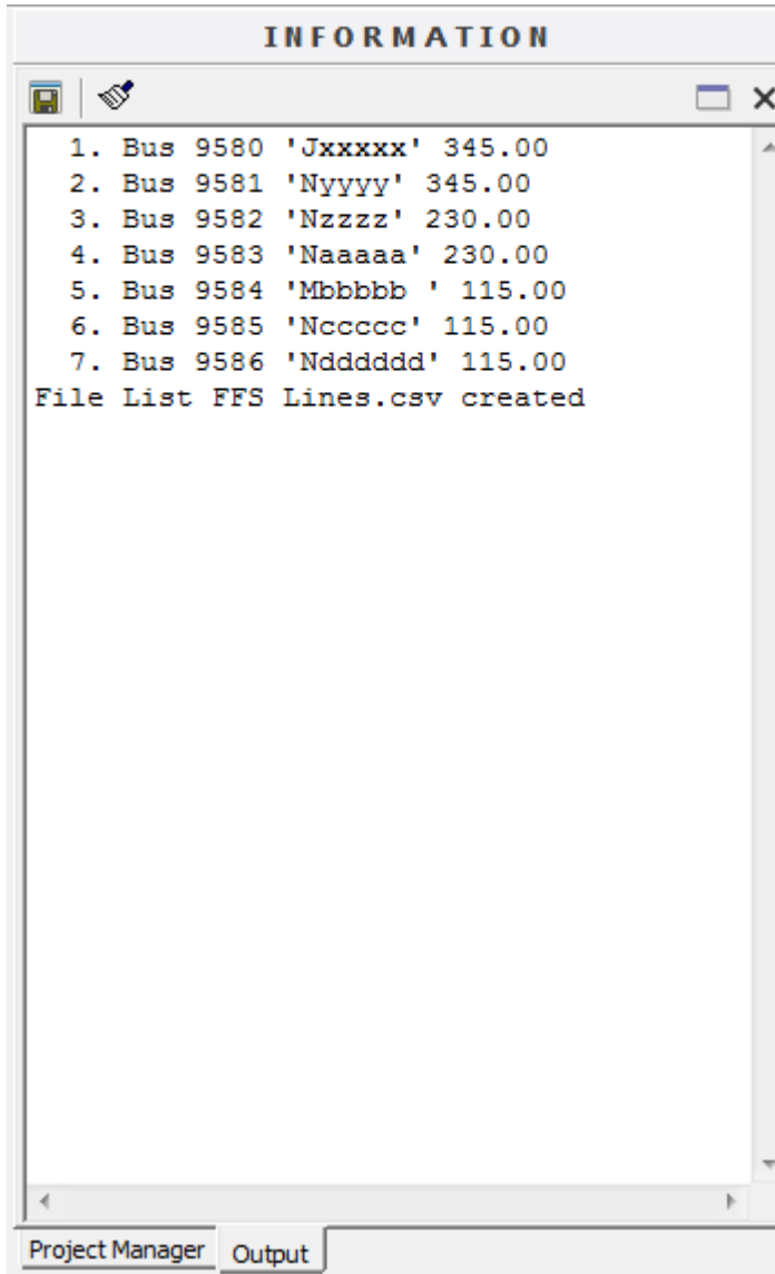
Figure 10-2. Output Tab during Execution of Activity “Determine Critical Buses”
