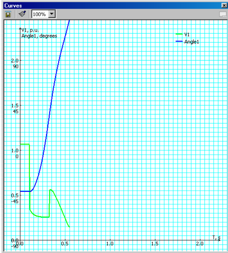
Figure 6-27. Fault at Bus # 138.0 Clears in 0.21 sec
