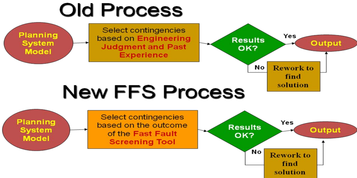
Figure 3-1. Transient Stability Assessment Process (Figure courtesy of Mr. Samrat Datta, Entergy Services)
