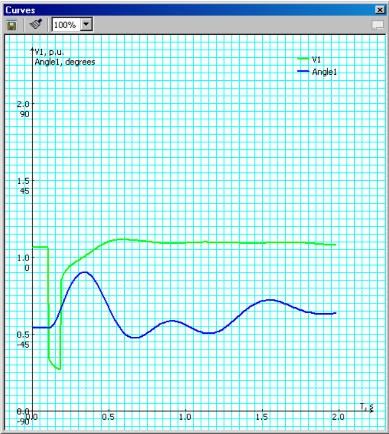
Figure 6-25. Fault at Bus # 138.0 Clears in 0.08 sec
