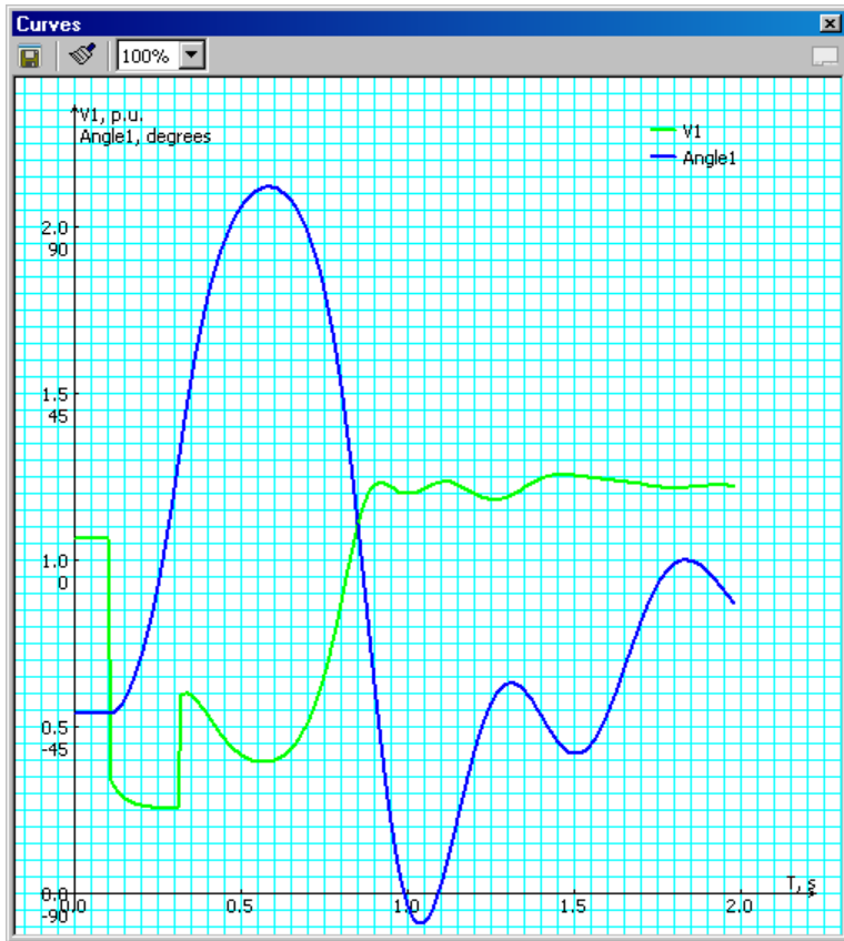
Figure 6-26. Fault at Bus # 138.0 Clears in 0.20 sec
